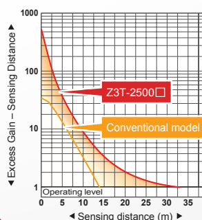
Excess Gain – Sensing Distance
